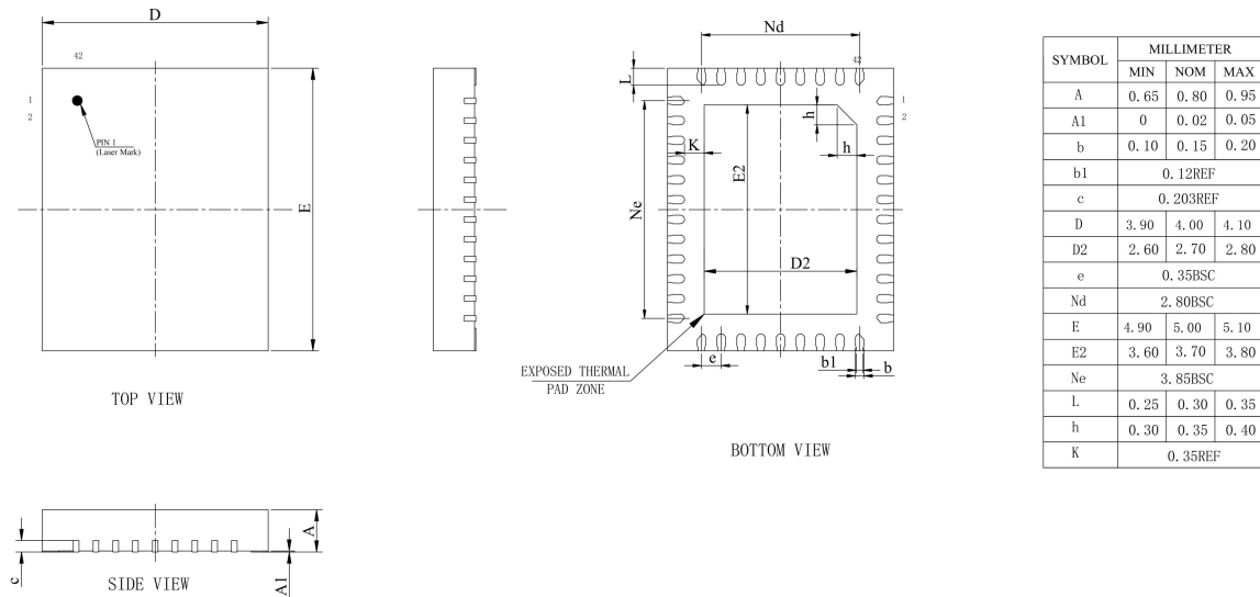
Figure 4-1 JL7083E Package
